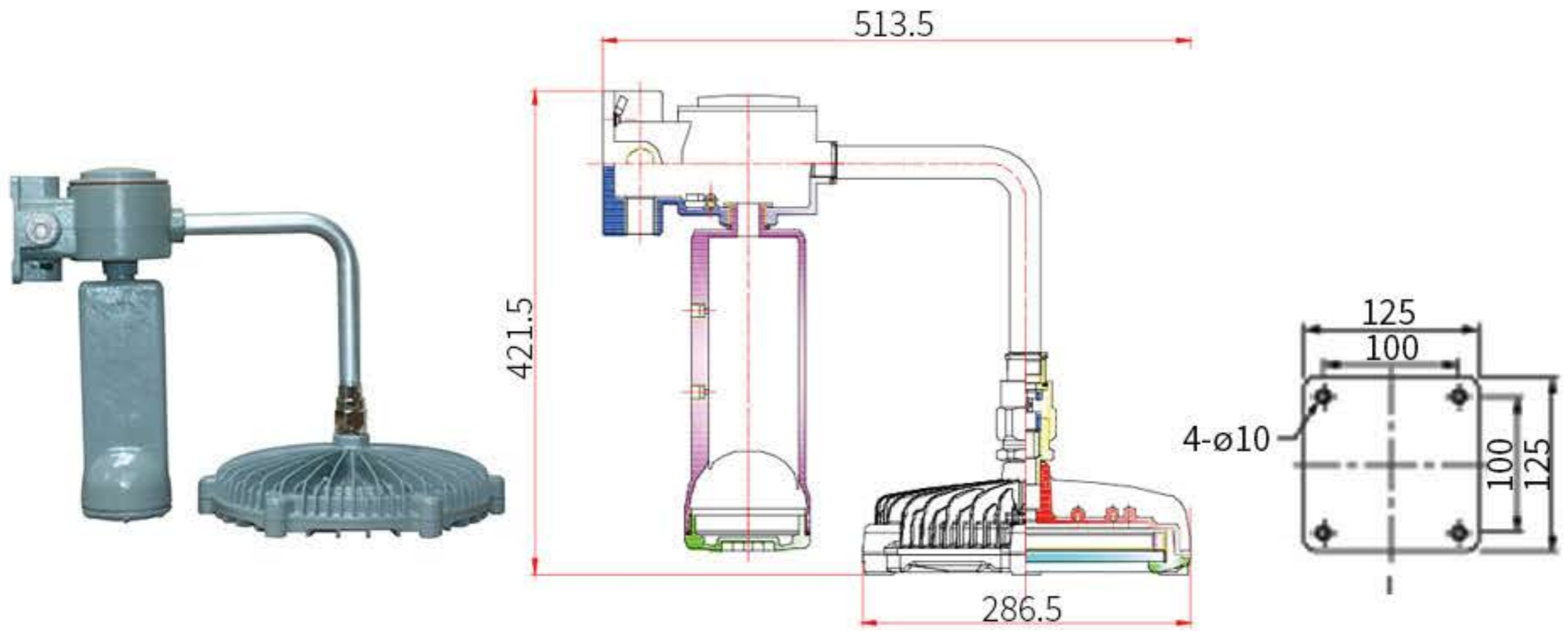
90° Bracket Type
